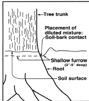
Figure 1. Placement Tide Paclo 2SC as basal drench
